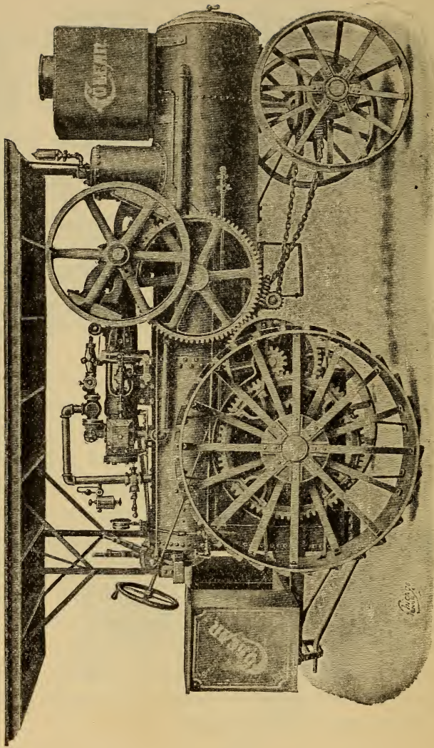
FIG. 35.—THE COLEMAN TRACTION ENGINE.
